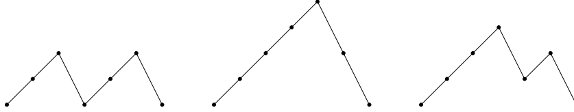
Fig. 1: Lattice paths corresponding to 1212, 1234, 1232.
