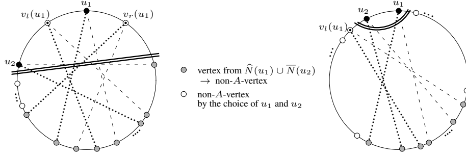
Fig. 2: Extended non-neighborhood \widehat{N}(u_1) and non-neighborhood \overline{N}(u_2) intersect
