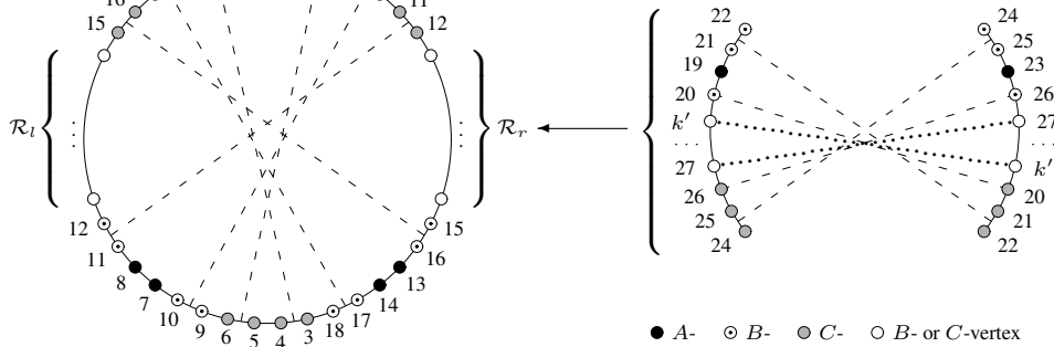
Fig. 5: b -coloring by k' = (2Q-1)3l + R + m colors (here for l = Q = 2, m = 1 )
