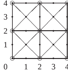
Fig. 4: The connectedness graph of v .
