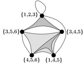
Fig. 1: Hypergraph associated to S = \{\{1, 2, 3\}, \{3, 4, 5\}, \{1, 4, 5\}, \{4, 5, 6\}, \{3, 5, 6\}\} . Number 2 appears only once in S so there is a loop attached to \{1, 2, 3\} . There are two edges of cardinality 2 determined by numbers 1 and 6, two edges of cardinality 3 since numbers 3 and 4 appear in three vertices of S , and one edge of cardinality 4 determined by number 5.
