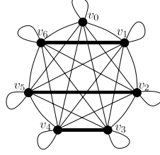
Fig. 4: The selected edges form the set \mathcal{E}_0 in \mathcal{H}_{7,7} .
