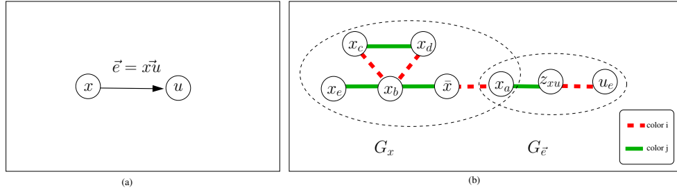
Fig. 6: (a) Arc \vec{e} = \vec{xu} of A , (b) Gadgets G_x and G_{\vec{e}} associated with vertex x and arc \vec{e} , respectively.
