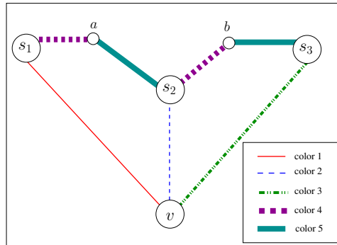
Fig. 3: Graph G_v^{c'} with endpoints S = \{s_1, s_2, s_3\} . The PEC paths \rho_1 and \rho_2 , respectively, with V(\rho_1) = (s_1, a, s_2) and V(\rho_2) = (s_2, b, s_3) are S -restricted while the PEC path \rho_3 with V(\rho_3) = (s_1, a, s_2, b, s_3) is non S -restricted.
