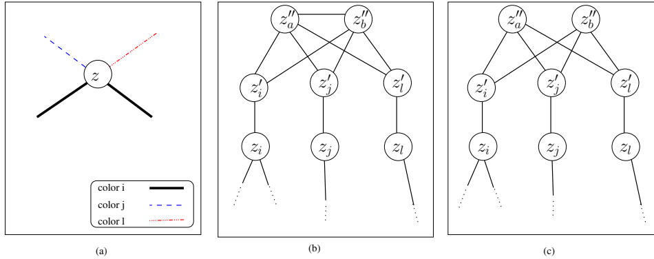
Fig. 2: (a) Vertex z of S_x in H^c(I_\alpha) ; (b) Gadget H_z associated to z \in S_x \setminus S'_x (c) Gadget H'_z associated to z \in S'_x .
