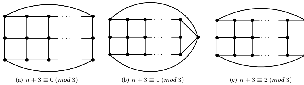
Fig. 2: The planar Ramsey graphs of order n + 3 for n \geq 8 .
