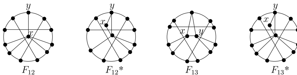
Fig. 6: Smallest xy -MNT graphs of order 12 (19 edges) and order 13 (21 edges)
