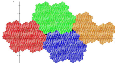
Fig. 4: Tiles \mathcal{T} , T_{011} , T_{001} and T_{100011}
