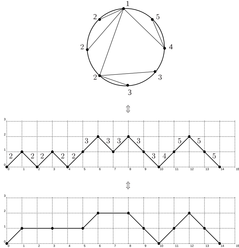
Fig. 2: The bijection between \text{GNC}_n(h, d) and \mathcal{S}_n .
