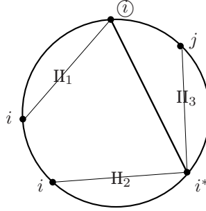
Fig. 3: The decomposition of Part II in (iii).
