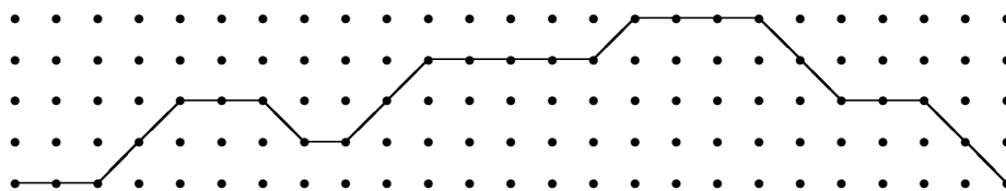
Fig. 2: A Motzkin path with \text{MinPlateau} = 2 , \text{MaxPlateau} = 3 , \text{MinLevel} = 1 and \text{MaxLevel} = 4 .
