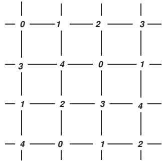
L(1,1) -labeling of G_4
