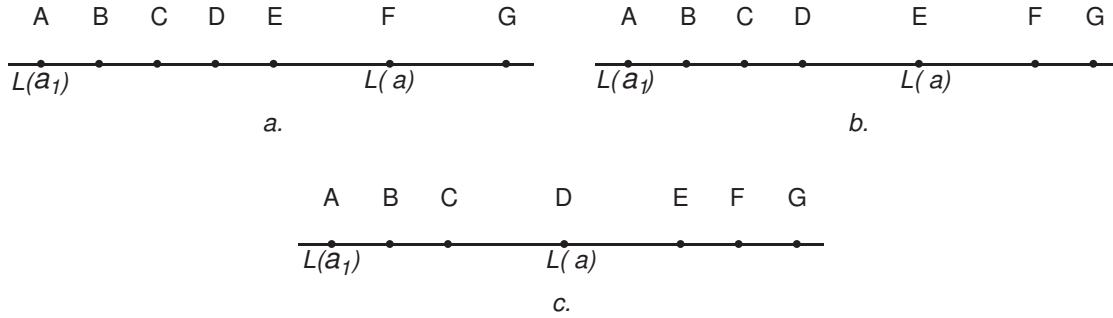
Fig. 8: Some possible relative positions of L(a) and of labels of a' neighbors.
