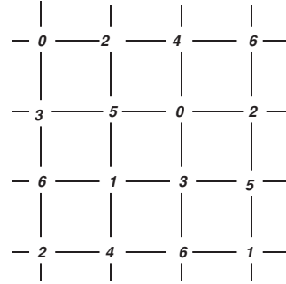
L(2,1) -labeling of G_4
