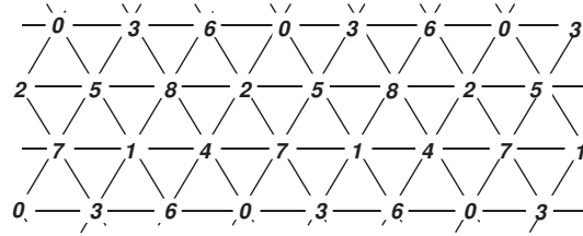
L(2,1) -labeling of G_6
