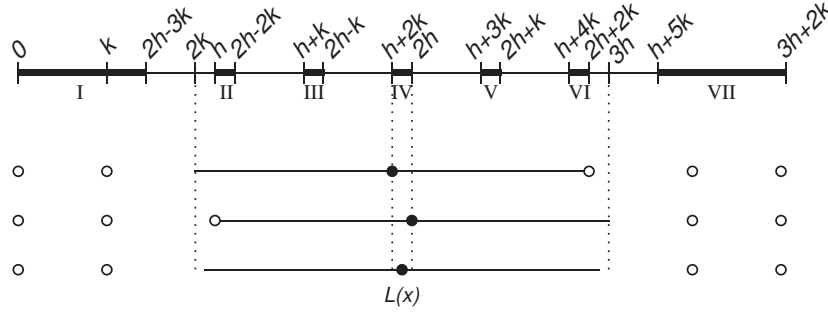
Fig. 9: The feasible intervals in the proof of Theorem 3.3.
