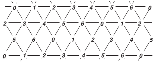
L(1,1) -labeling of G_6
