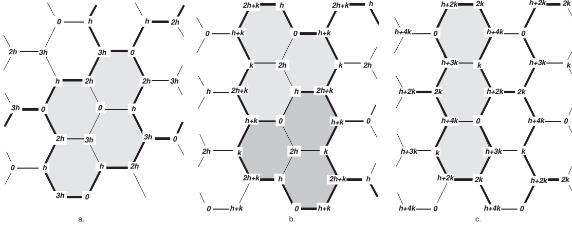
Fig. 10: Three optimally labeled portions of hexagonal grid, when a. k \leq h \leq \frac{5}{3}k , when b. 2k \leq h \leq 3k and when c. h \geq 3k .
