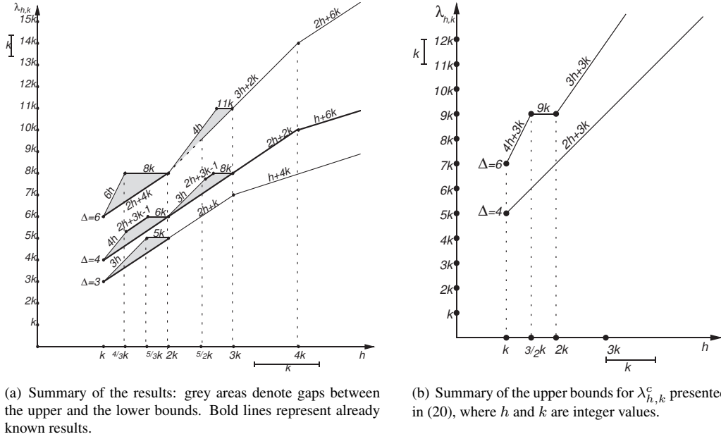
Fig. 2: Summaries of bounds.
