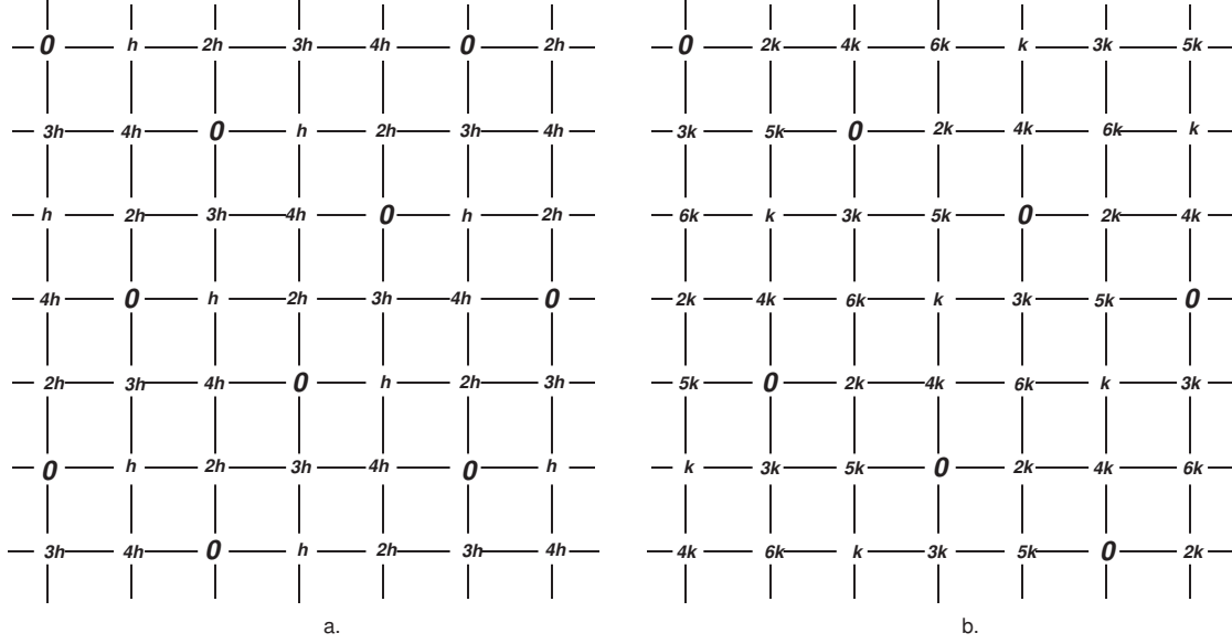
Fig. 11: Two optimally labeled portions of squared grid, when a. k \leq h \leq \frac{3}{2}k and when b. \frac{3}{2}k \leq h \leq 2k .
