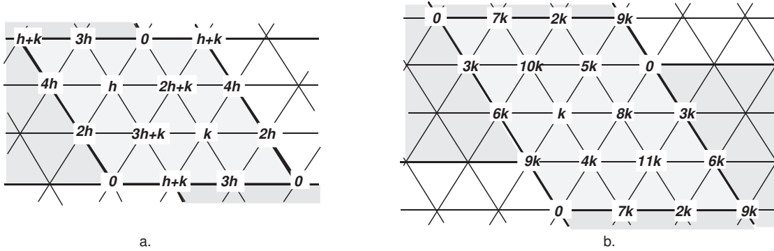
Fig. 6: Two feasible labelings of a cellular graph when 2k \leq h \leq 3k . Their span is a. 4h and b. 11k .
