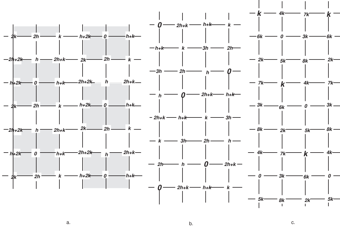
Fig. 12: a. and b. two feasible L(h, k) -labelings when 2k \leq h \leq \frac{8}{3}k and when \frac{8}{3}k \leq h \leq 3k .
