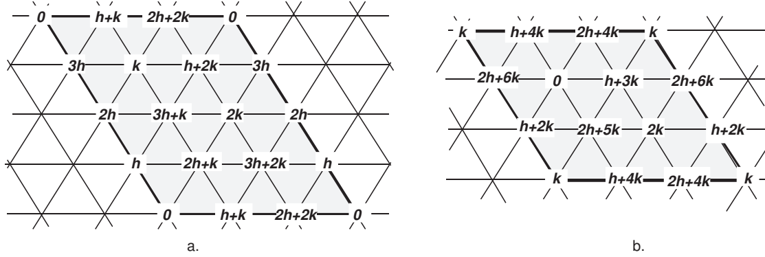
Fig. 7: Two optimally labeled portions of cellular graph when a. 3k < h < 4k and b. h \geq 4k .
