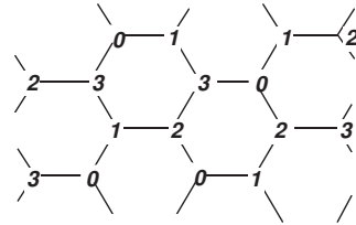
L(1,1) -labeling of G_3
