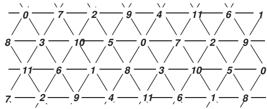
L(3,1) -labeling of G_6
