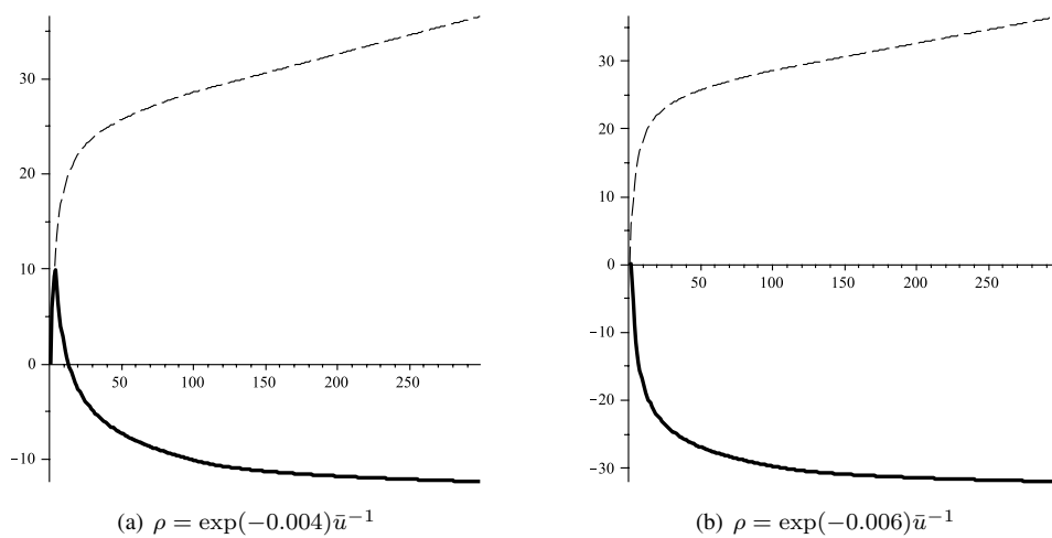
Fig. 10: Actual potential (dashed) and apparent asymptotic potential (plain) for a concave walk with p_n = 0.48 \exp(-\frac{100}{n^2}) , N = 100 and t = 10,000 .
