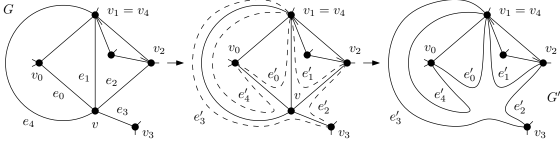
Fig. 2.1. The annihilation of a vertex v . The original graph G is on the left, the resulting graph G' on the right.
