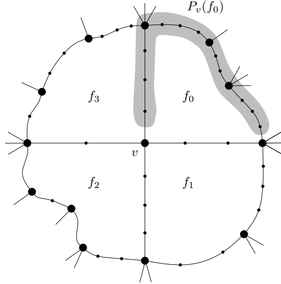
Fig. 2.2. The definition of the path P_v(f_i) for i = 0 and a vertex v of degree 4. High-degree vertices are shown as larger dots.
