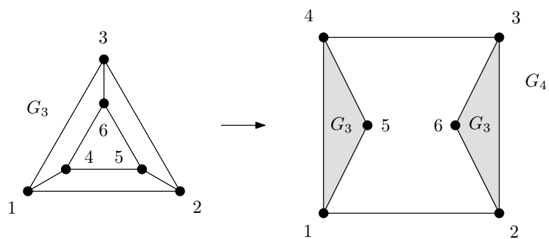
(b) The graphs G_3 (left) and G_4 (right).
