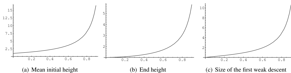
Fig. 2: Mean initial height, end height and size of the first weak descent as a function of q .
