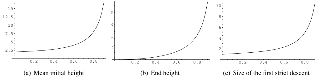
Fig. 1: Mean initial height, end height and size of the first strict descent as a function of q .
