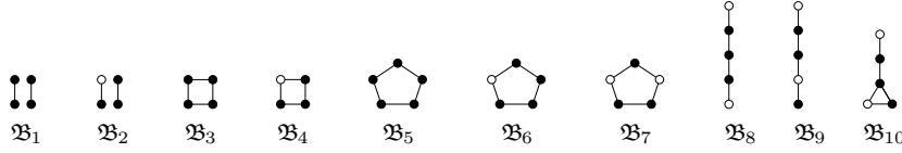
Fig. 2: Forbidden subgraphs for partitioned probe split graphs (black vertices probes, white vertices non-probes).
