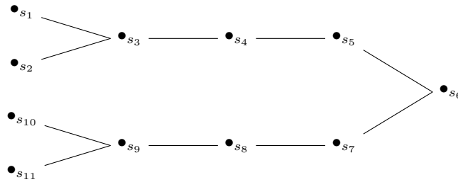
Fig. 1: The Coxeter graph of \tilde{D}_{11} with root s_6 , corresponding to the reflection t = s_1 s_2 \cdots s_5 s_{10} s_{11} s_9 s_8 s_7 s_6 s_7 s_8 s_9 s_{11} s_{10} s_5 \cdots s_2 s_1 .
